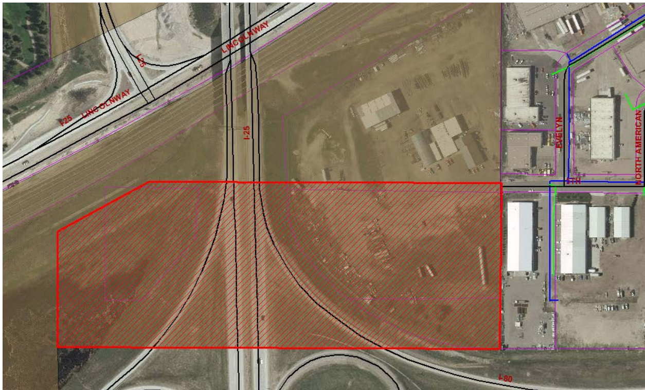
Water lines in blue; sewer in green.
